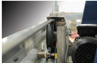
Rollers Inside Bridge and trolley movements are smooth and effortless using internally mounted dual-axis rollers. The hanging design enhances self-centering and improved roller life by protecting the rollers from the harsh wash environment.
